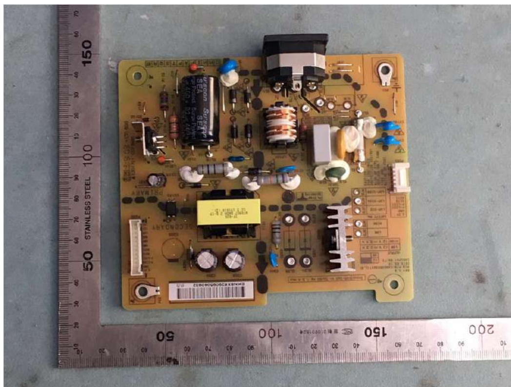
FIGURE 12 LCD MONITOR (M/N: 24BN650U) POWER BOARD (COMPONENT SIDE)
