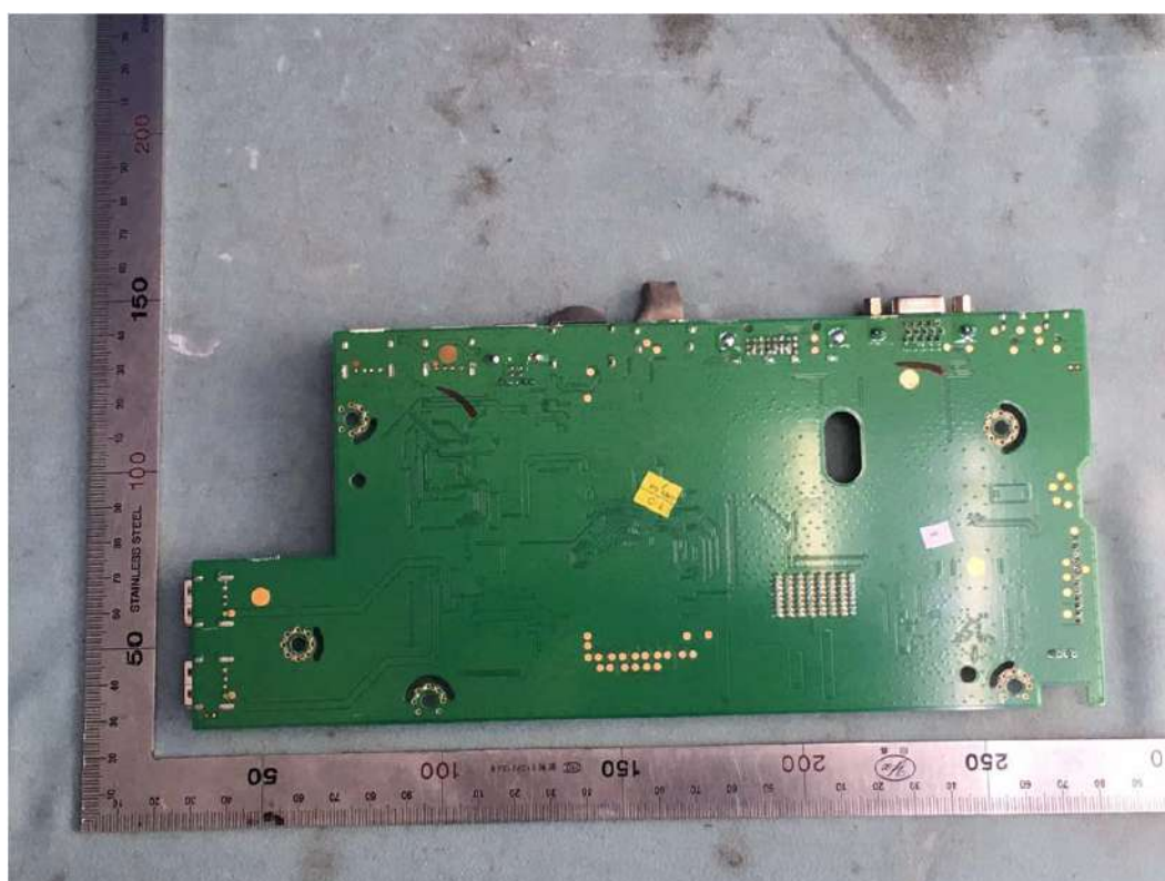
FIGURE 9 LCD MONITOR (M/N: 24BN650U) MAIN BOARD (SOLDERED SIDE)
