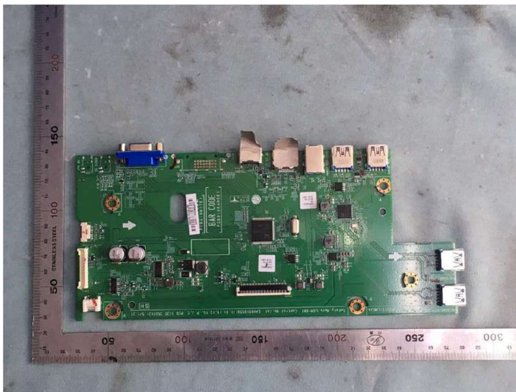
FIGURE 9 LCD MONITOR (M/N: 24BN650U) MAIN BOARD (COMPONENT SIDE)
