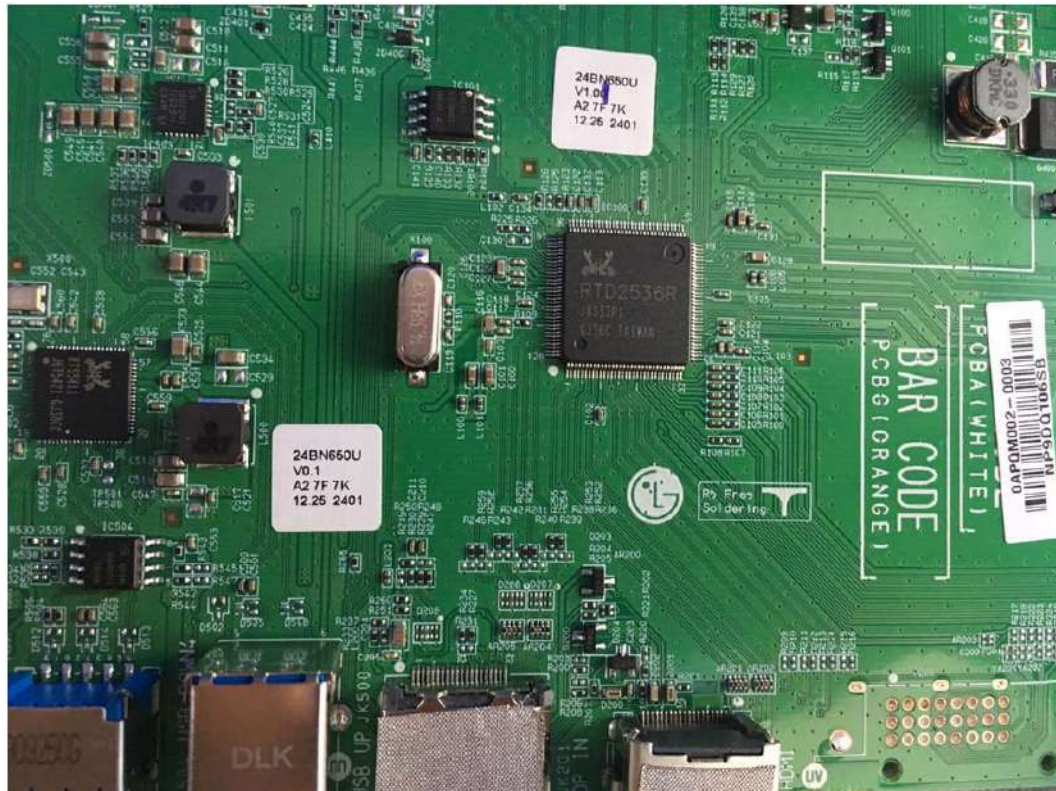
FIGURE 10 LCD MONITOR (M/N: 24BN650U) CRYSTAL AND CHIP ON MAIN BOARD
