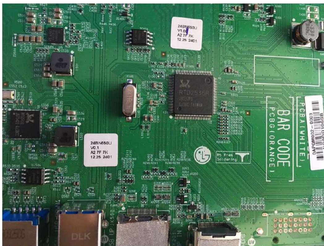
FIGURE 11 LCD MONITOR (M/N: 24BN650U) CRYSTAL AND CHIP ON MAIN BOARD
