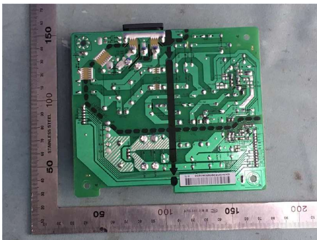
FIGURE 13 LCD MONITOR (M/N: 24BN650U) POWER BOARD (SOLDERED SIDE)
