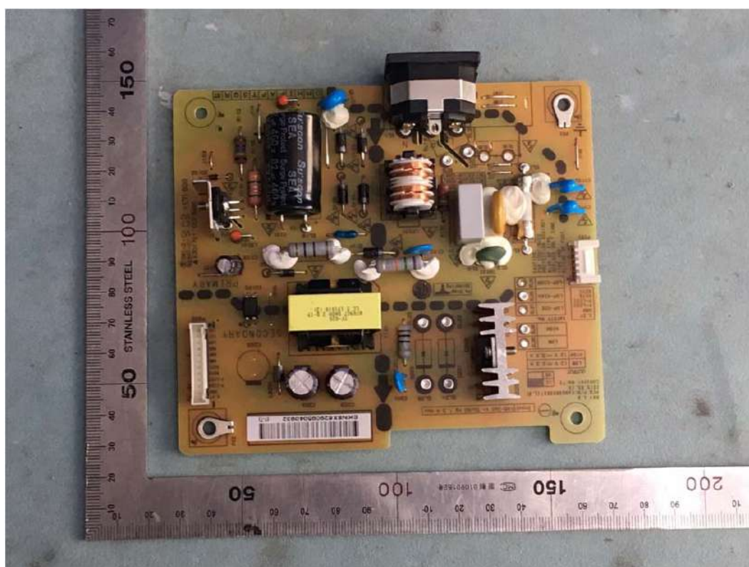
FIGURE 11 LCD MONITOR (M/N: 24BN650U) POWER BOARD (COMPONENT SIDE)
