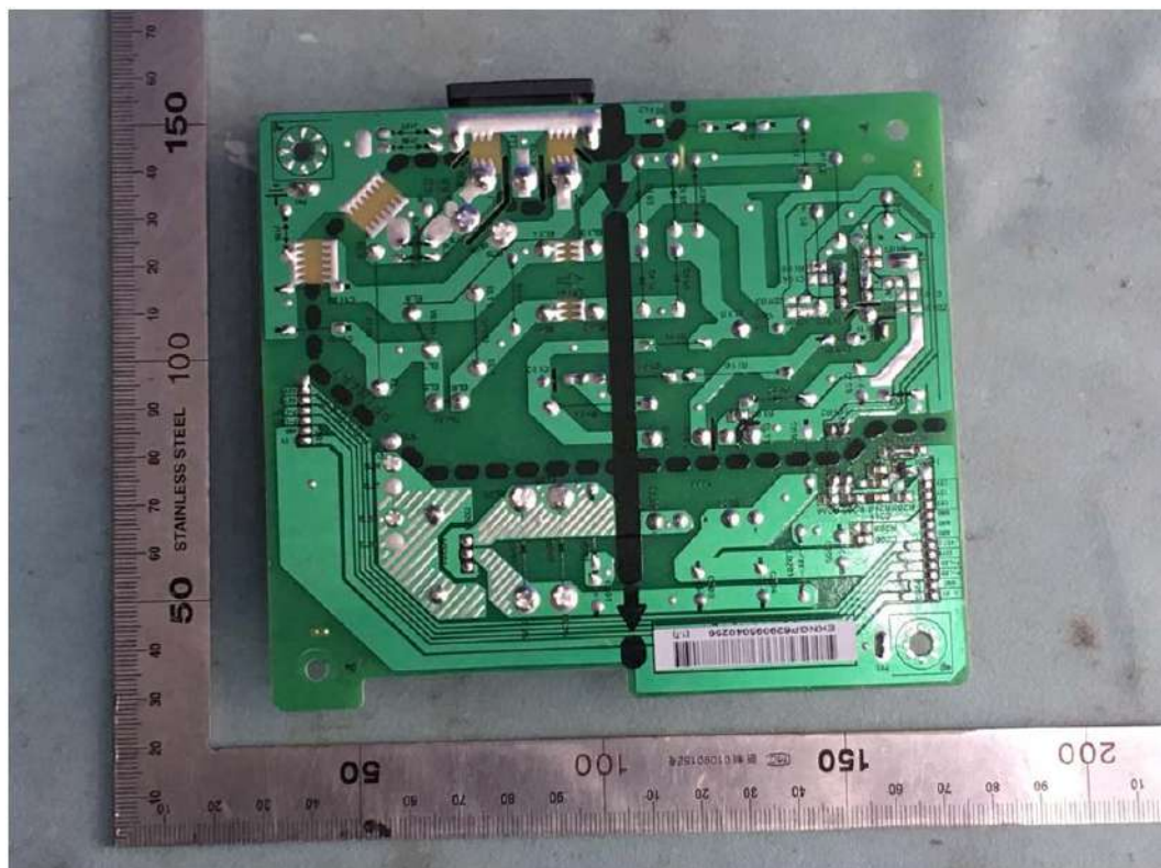
FIGURE 12 LCD MONITOR (M/N: 24BN650U) POWER BOARD (SOLDERED SIDE)
