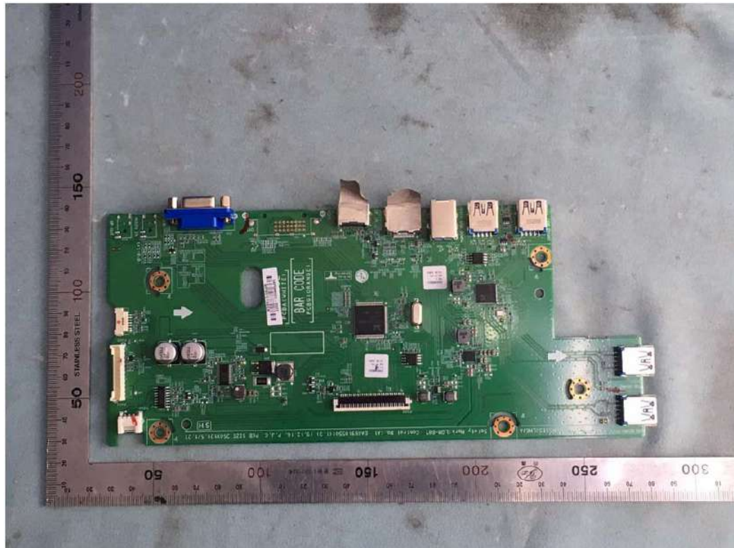
FIGURE 8 LCD MONITOR (M/N: 24BN650U) MAIN BOARD (COMPONENT SIDE)
