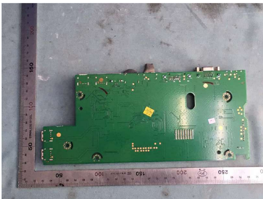
FIGURE 10 LCD MONITOR (M/N: 24BN650U) MAIN BOARD (SOLDERED SIDE)
