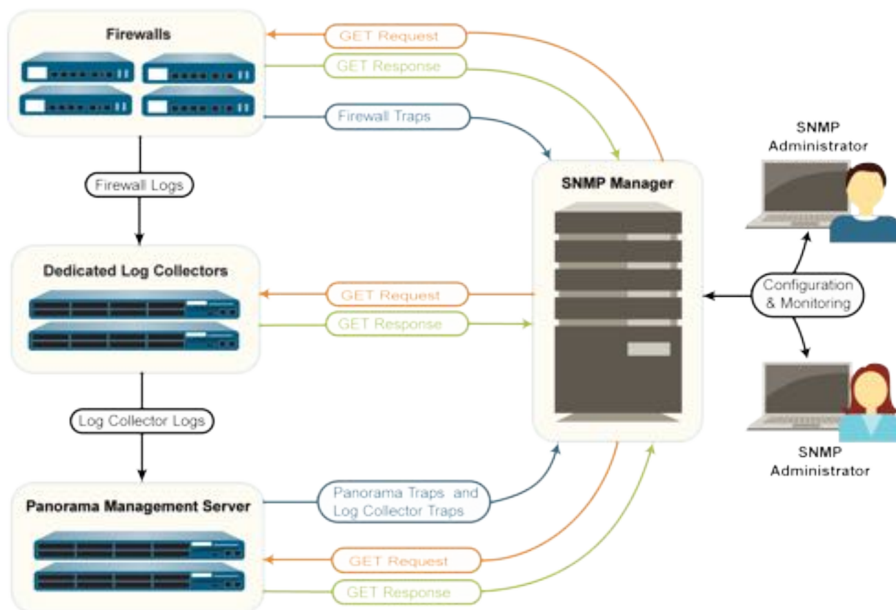
Figure 2: SNMP Implementation
